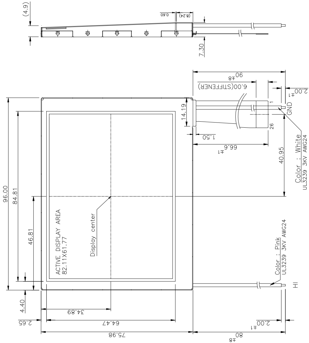
Fig.1 Outline dimension of TFT-LCD module
